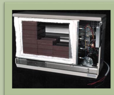
ETS Room Unit (cutaway view)
